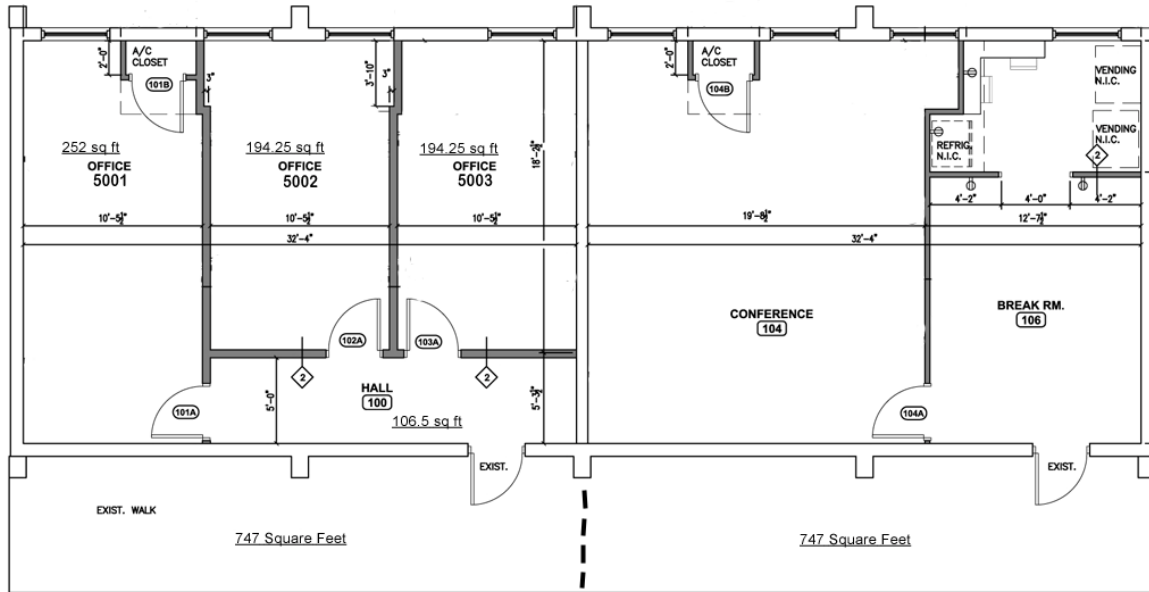
1 Bldg. 5 FLOOR PLAN SCALE: 1/4" = 1'-0"
